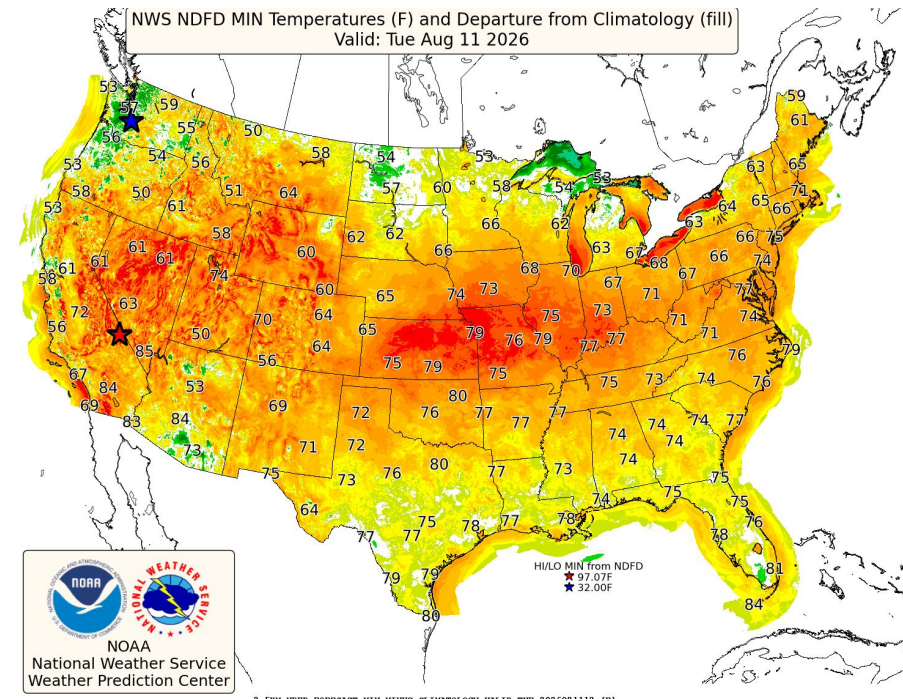
Tomorrow Night
