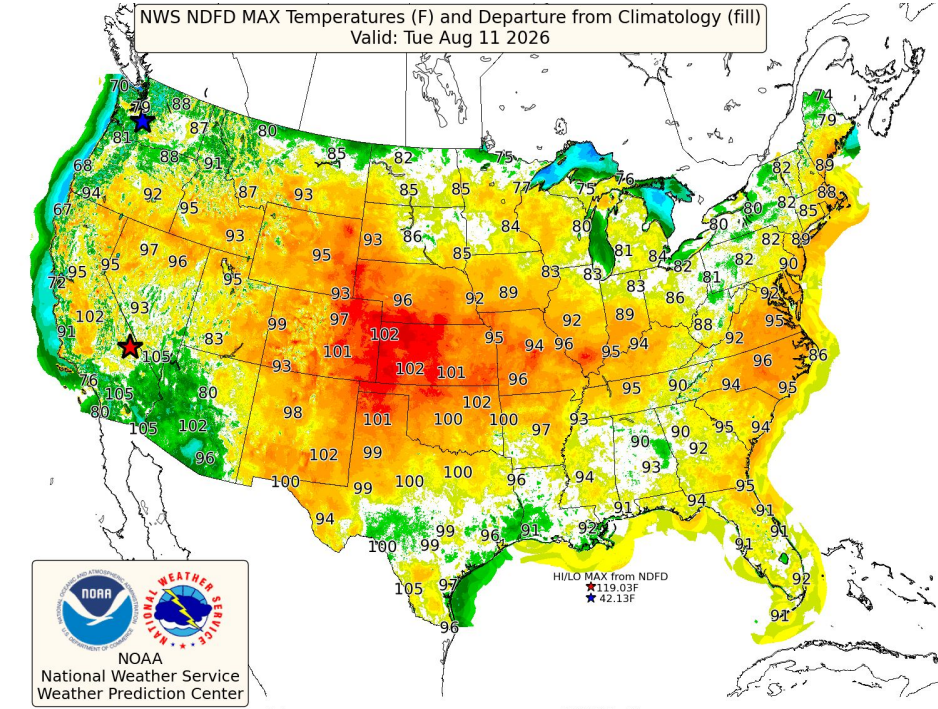
Day 3
