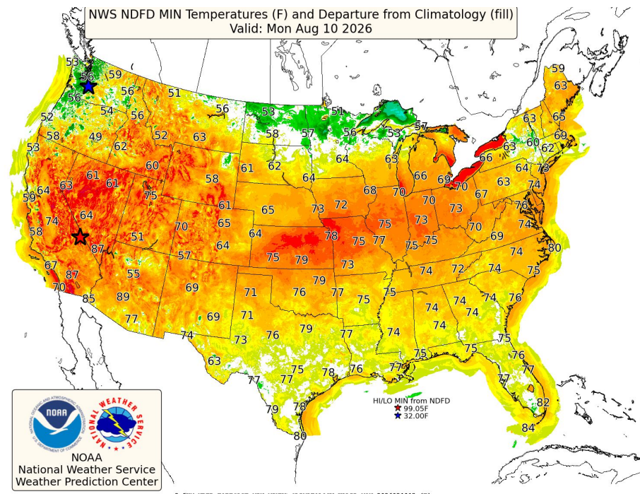
Tonight
